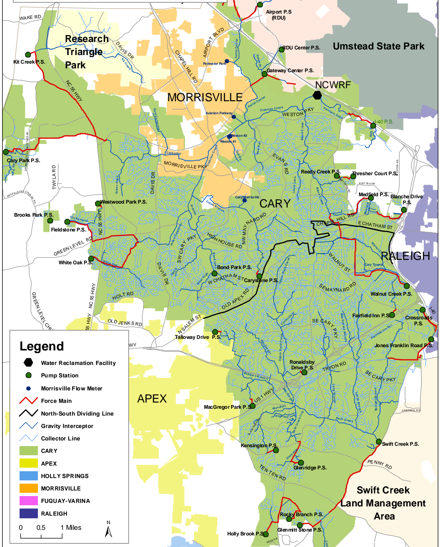
Figure 3-2 Town of Cary Existing Wastewater Collection System
