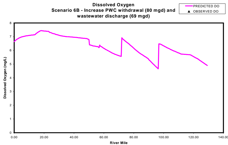
FIGURE 6-2B. Buckhorn Dam to Lock and Dam 1 Predicted Dissolved Oxygen for Select Scenarios without Phytoplankton Productivity
