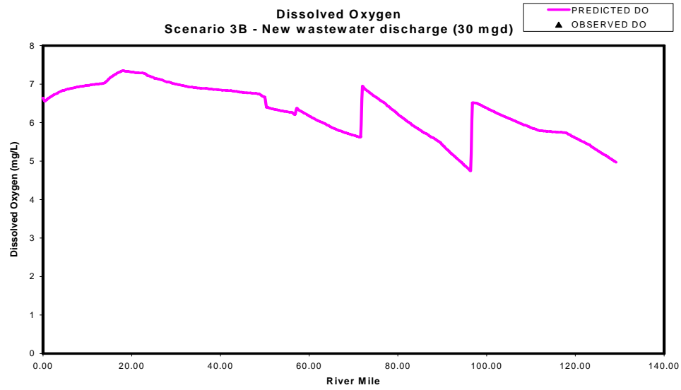
FIGURE 6-2A. BUCKHORN DAM TO LOCK AND DAM 1 Predicted Dissolved Oxygen for Select Scenarios without Phytoplankton Productivity
